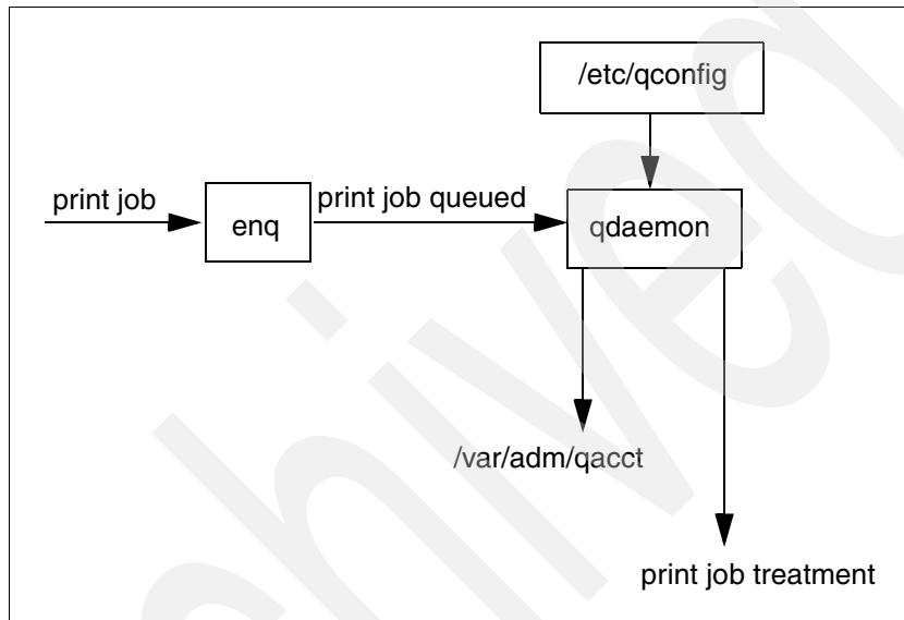
Figure 3-4 Generating print accounting data
