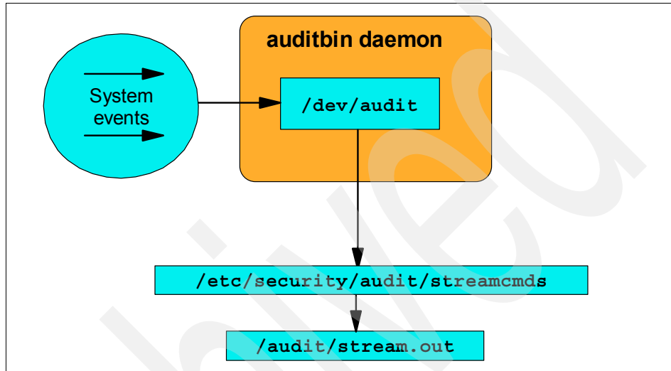
Figure 2-3 Data collection in STREAM mode
