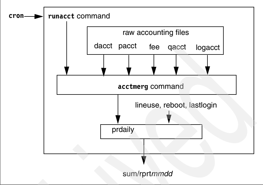
Figure 3-5 Generating daily accounting reports
