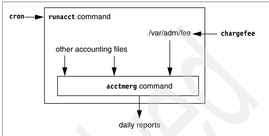
Figure 3-13 Generation and merging fee report
