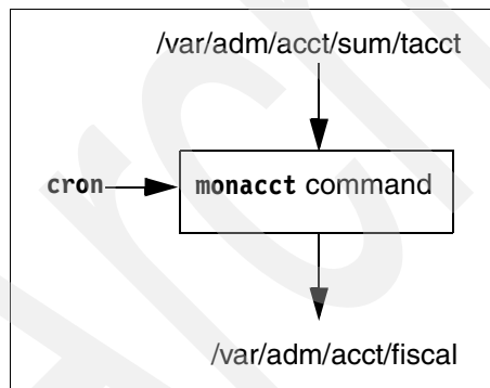
Figure 3-7 Generate the monthly (fiscal) reports
