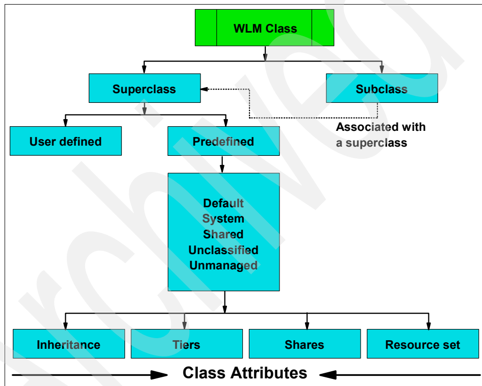
Figure 4-1 WLM class concept diagram
