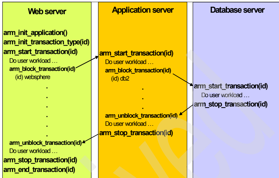
Figure 5-3 ARM API calls
