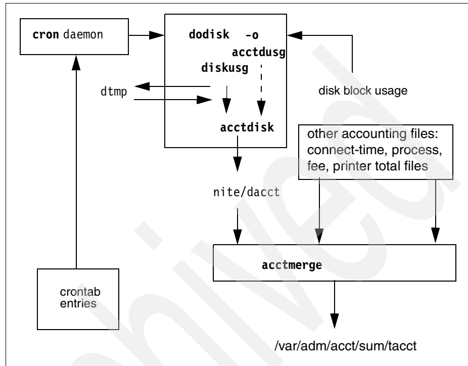
Figure 3-3 Collecting disk block accounting data
