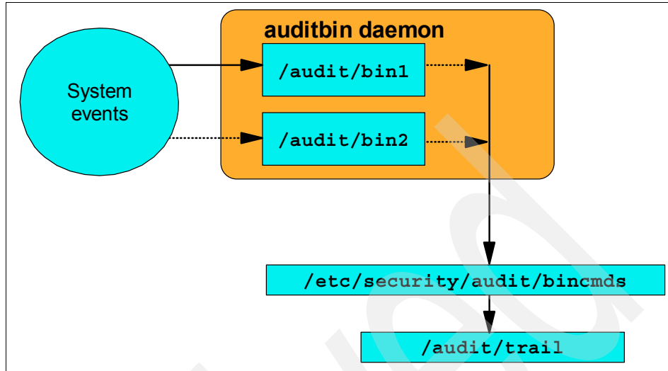
Figure 2-2 Data collection in BIN mode
