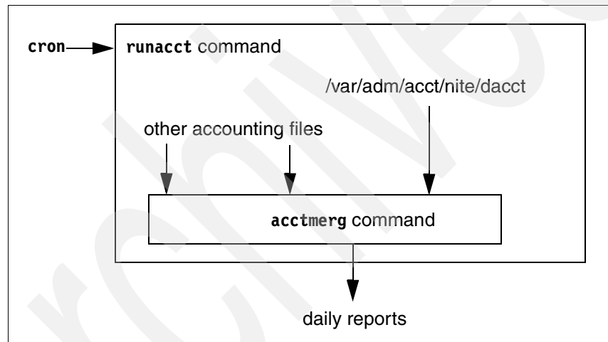
Figure 3-11 Generation and merging of disk-usage report
