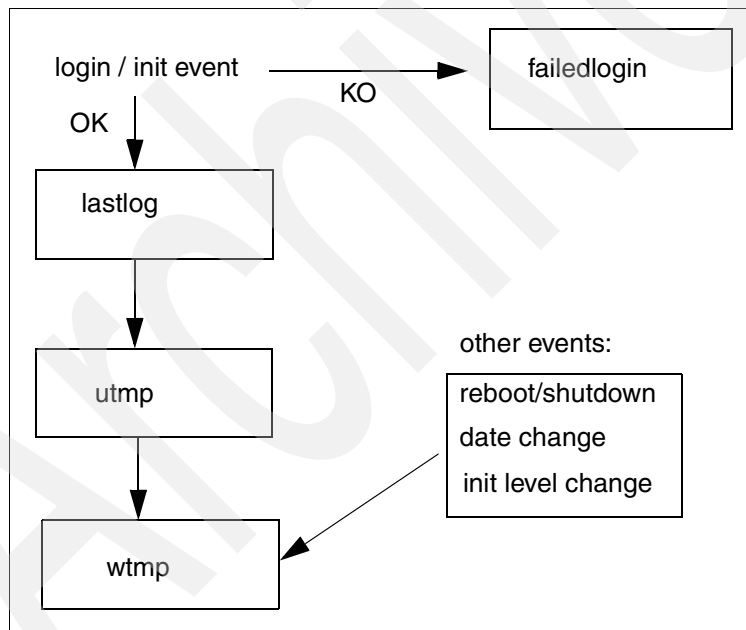
Figure 3-2 Connect-time accounting process
