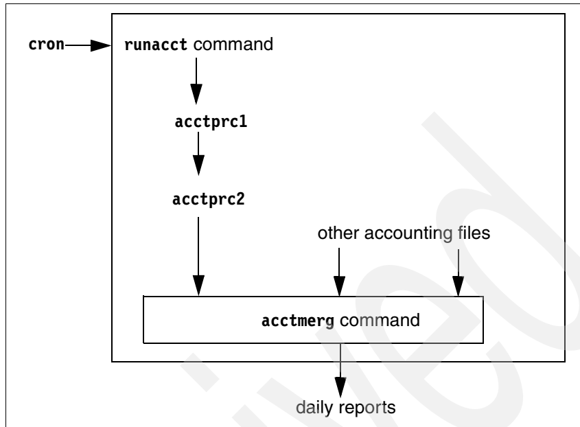
Figure 3-10 Generation and merging of process report
