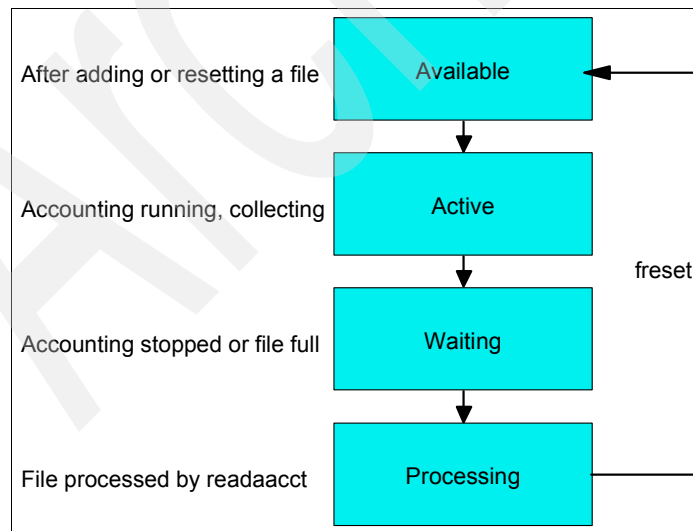
Figure 5-2 Status of accounting files
