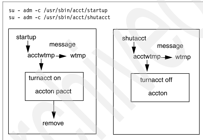
Figure 3-1 How the startup and shutacct commands work
