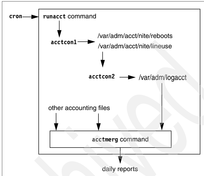
Figure 3-9 Generation and merging of connect-time report
