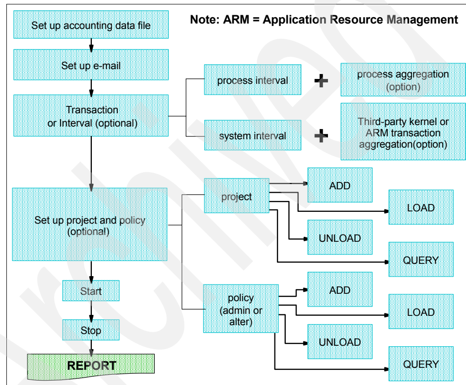
Figure 5-1 Advanced accounting setup overview
